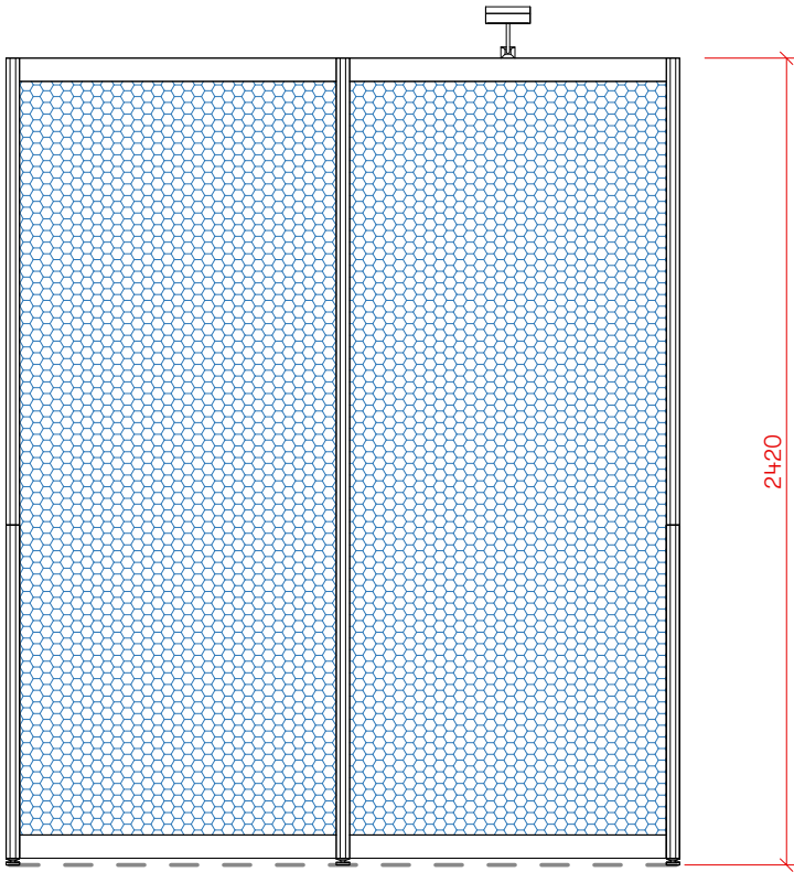
2 Elevation - Front A03 1 : 25
